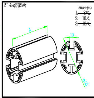
B2062C 2" 鋁套管3向10尺銀
