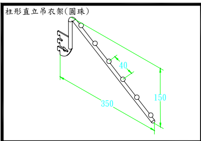
D0010C 柱形直立吊衣架(圓珠)銀
