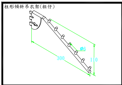
D0070C 柱形傾斜吊衣架(粒仔)銀
